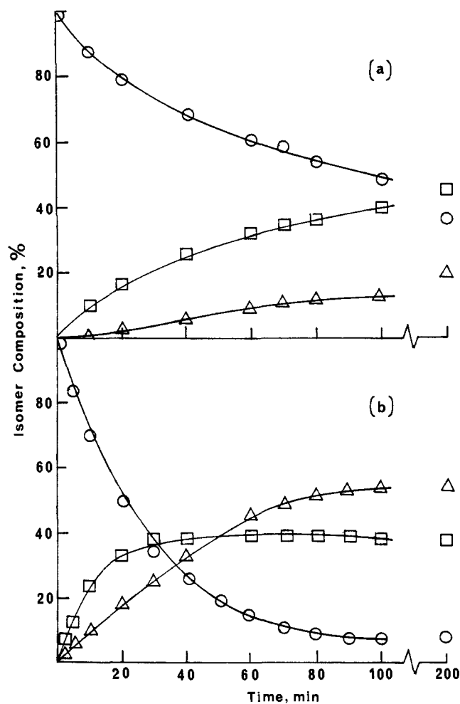
Figure 5. Composition of the isomer mixture vs. irradiation time for isomerization of 0.01 M ( E,E )- 12 (○) to ( E,Z )- 12 (□) and ( Z,Z )- 12 (△) in the absence (a) and presence (b) of 0.01 M \text{BF}_3 \cdot \text{OEt}_2 .
