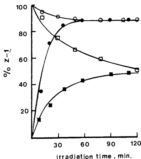
Figure 1. Formation of ( Z )-1 upon irradiation of ( E )-1 in the absence (■) and presence (●) of \text{BF}_3 \cdot \text{OEt}_2 and the disappearance of ( Z )-1 upon irradiation in the absence (□) and presence (○) of \text{BF}_3 \cdot \text{OEt}_2 .
