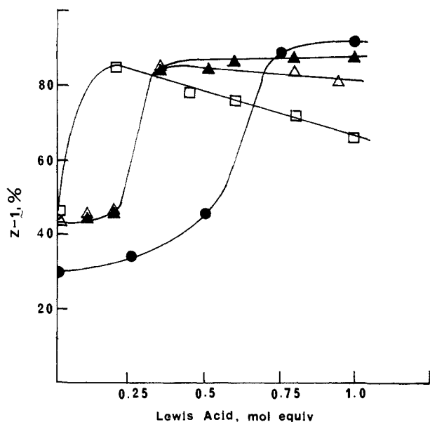
Figure 3. Solvent dependence of the optimum conversion of ( E )-1 to ( Z )-1 in the presence of \text{AlCl}_3 (empty symbols) and \text{EtAlCl}_2 (filled symbols) in hexane (O), benzene ( \Delta ), and dichloromethane ( \square ) solutions.
