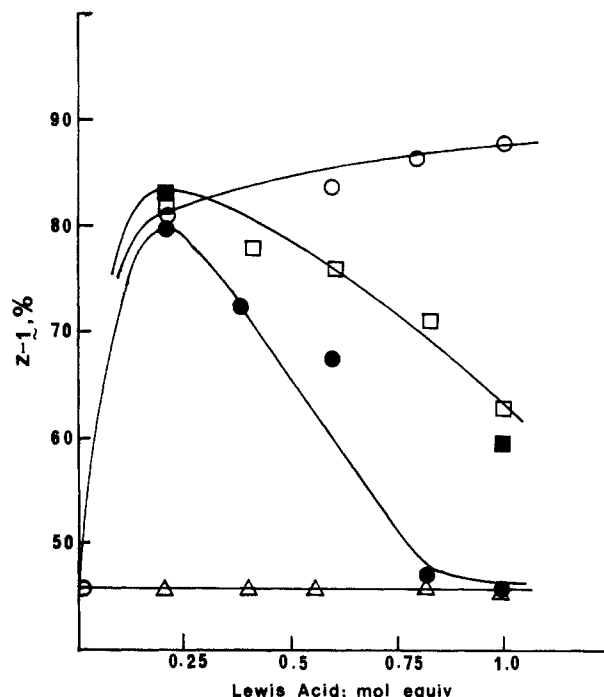
Figure 2. Effect of Lewis acid concentration on the optimum conversion of ( E )-1 to ( Z )-1 in the presence of \text{BF}_3 \cdot \text{OEt}_2 (○), \text{SnCl}_4 (●), \text{AlCl}_3 (□), \text{EtAlCl}_2 (■), and \text{ZnCl}_2 (△) in dichloromethane solution.
